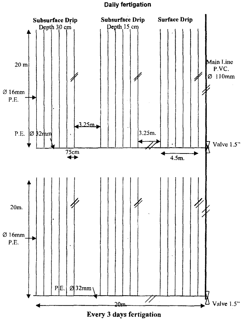
Fig. 1. Layout of the experiment.
