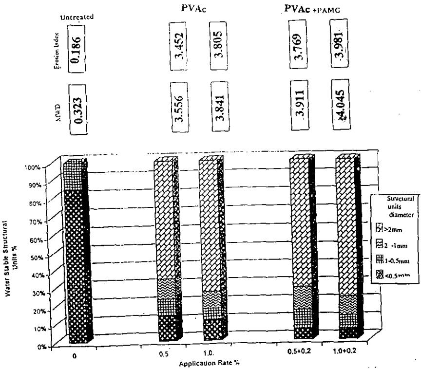
Fig. 1. Effect of conditioner type and rate of application on the distribution of water stable structural units and their MWD and erosion index for the Bourg El-Arab calcareous soil.
