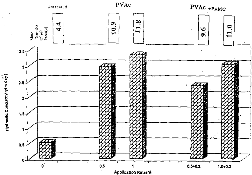
Fig. 4. Effect of conditioner type and rate of application on soil hydraulic conductivity (m day -1 ) and mean pore diameter (μ) of the Bourg El-Arab calcareous soil.
