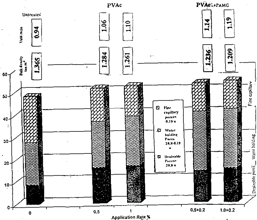
Fig. 2. Effect of conditioner type and rate of application on soil bulk density, void ratio, total porosity and pore size distribution of the Bourg El-Arab calcareous soil.
