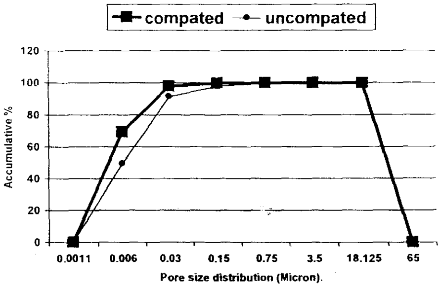
Fig. 2. Accumulative percentage of pore size distribution in compacted and uncompact soils.
