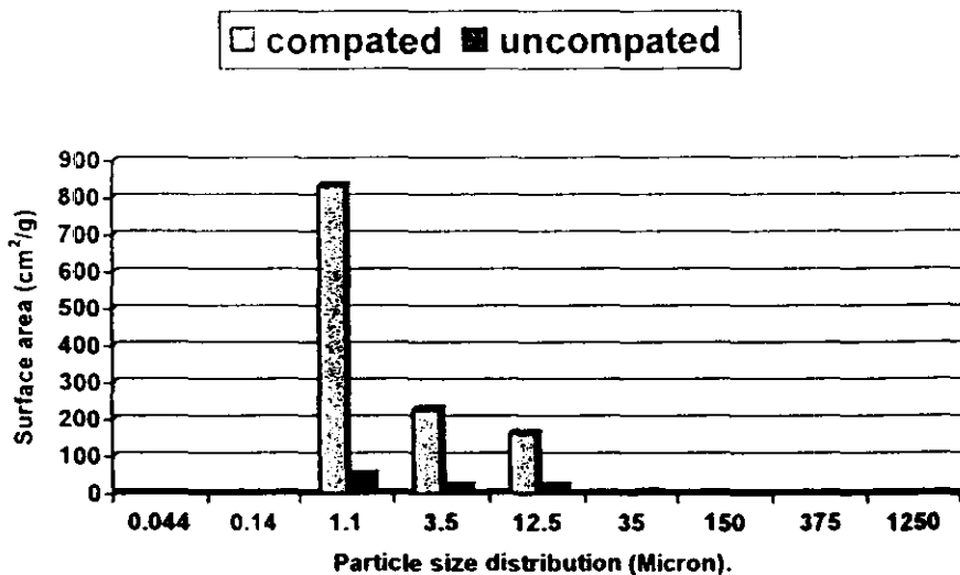
Fig. 6. The relationship between surface area ( \text{cm}^2/\text{g} ) and particle size distribution for compacted and uncompact soils.
