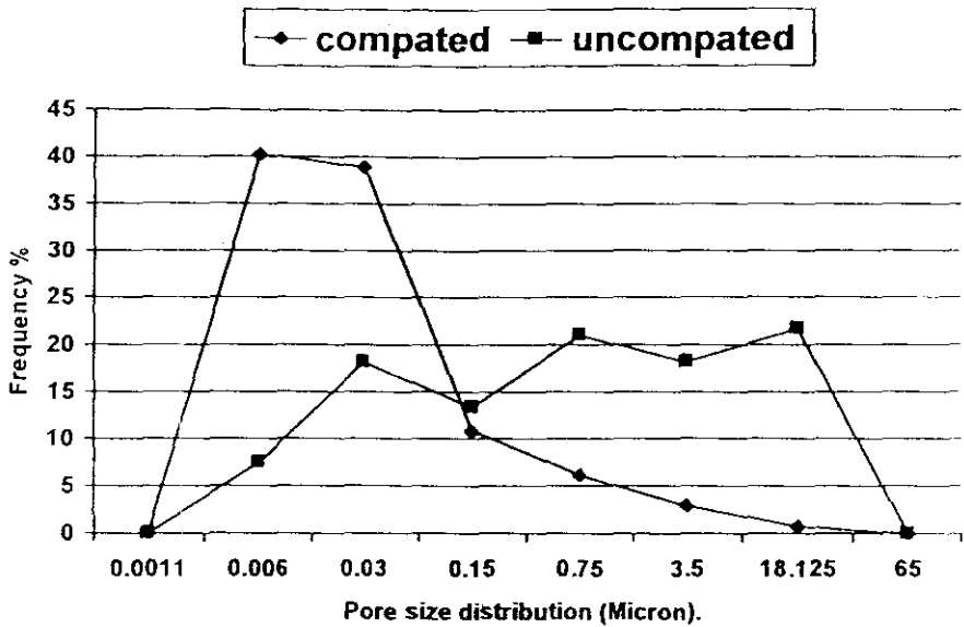
Fig. 1. Frequency percentage of pore size distribution in compacted and uncompact soils.
