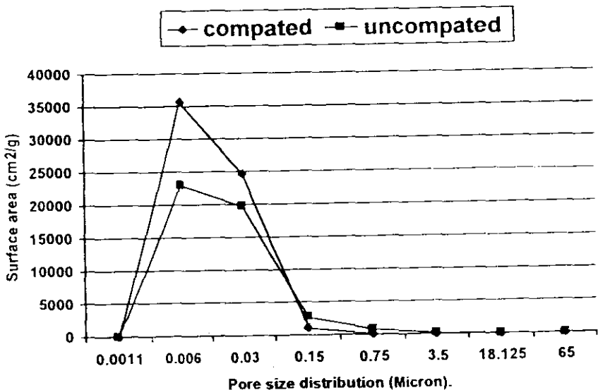
Fig. 3. The relationship between surface area ( \text{cm}^2/\text{g} ) and pore size distribution for compacteds and uncompacteds soils.
