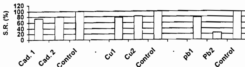
Fig. (3): Effect of cadmium, copper and lead on survival rate of Nile tilapia O. niloticus
