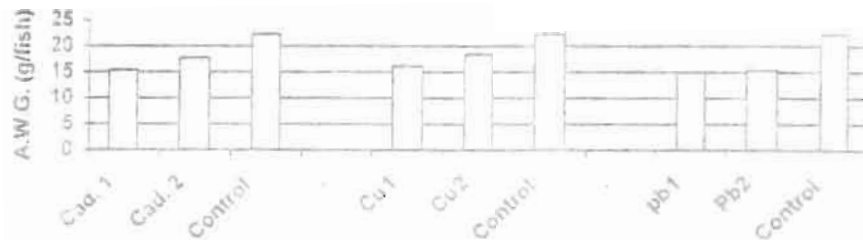
Fig. (1): Effect of cadmium, copper and lead on average weight gain of O. niloticus .
