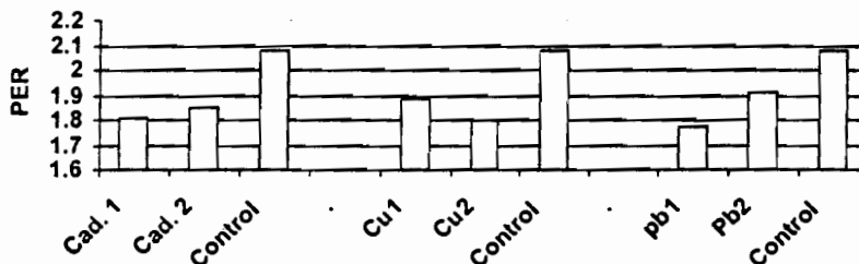
Fig. (5): Effect of cadmium, copper and lead on protein feed efficiency ratio in Nile tilapia ( Oreochromis niloticus ).
