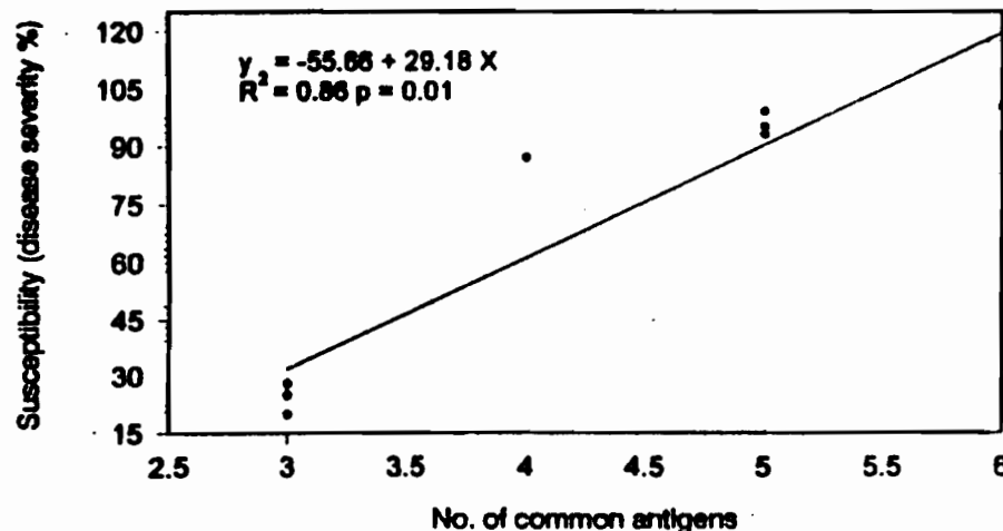
Fig. 2: Regression equation that describes the relationship between number of common antigens (x) found in Oidium lini -infected whole plants of flax cultivar Giza 8 and in seeds from healthy cultivars and susceptibility (Y) of these cultivar to O. lini .
