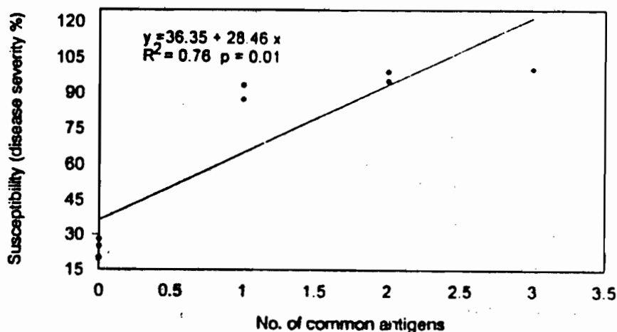
Fig. 3: Regression equation that describes the relationship between number of common antigens (X) found in Oldium lini and in seeds from healthy cultivars and susceptibility (Y) of these cultivar to O. lini .
