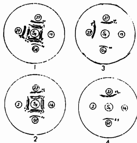
Fig (1). Diagram showing the double-diffusion reaction of antiserum ( S_2 ) of the infected whole plant of Giza 8 (1 and 2) and the antiserum ( S_1 ) of Oidium lini (3, 4) against antigens of seeds from eight healthy cultivars. Cultivars were: Cortland (22), Linore (27), C.I. 2008 (29), Dakota (2), Willden (14), Williston Brown (15), Giza 7 and Giza 8.
