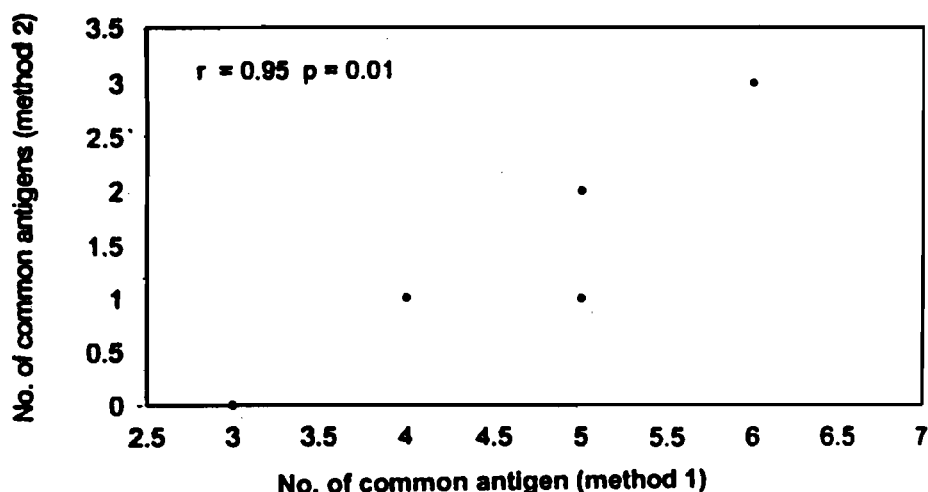
Fig. 4: Correlation between two methods used to study the antigenic relationship between Oidium lini and flax cultivars. In the first method, antiserum of whole flax plants of cultivar Giza 8 infected with O. lini interacted against antigens of seeds from healthy flax cultivars. In the second method, antiserum of O. lini interacted against antigens of seeds from healthy flax cultivars after elimination of Giza 8 antibodies from the antiserum of infected whole plants by reciprocal precipitation.
