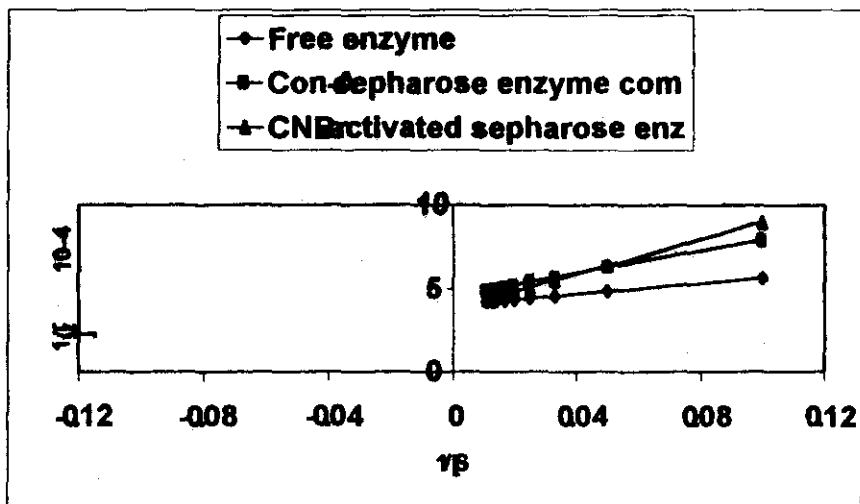
Fig. (4b): Lineweaver-Burk plots of free and immobilized invertase.
