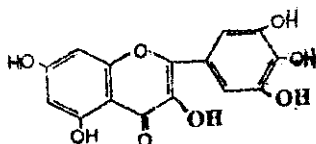
Myricetin
