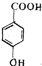
P-hydroxybenzoic acid.
