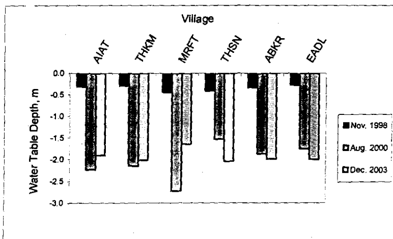
Figure (5): Average water table depths as before (November 1998) and after the installation of the main drain. (Ali Ibn Abi Taleb=AIAT, Mohamed Refaat=MRFT, and Tawfeek El-Hakeem=THKM), and three other villages (Abou Bakr=ABKR, El-Adl=EADL, and Taha Hussein=THSN) in the vicinity of Bustan 1 and 2.
