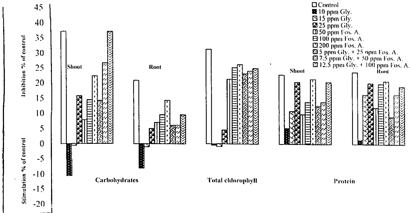
Fig (1): Herbicidal effect of glyphosate, fosamine ammonium and their mixture on some chemical composition in pea plant at different concentrations.
