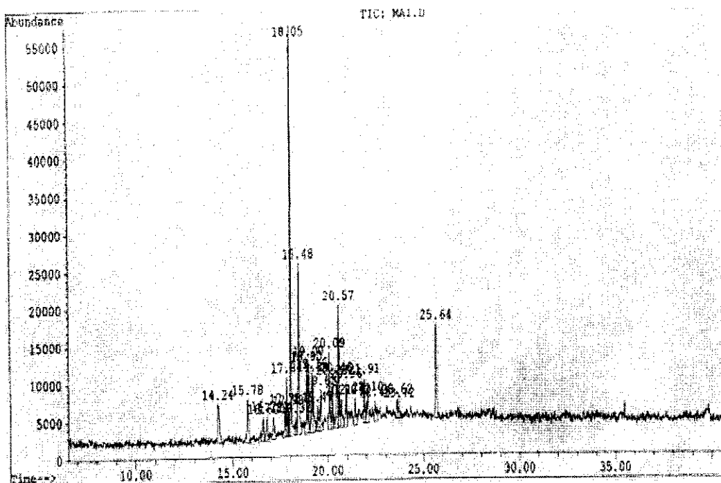
Fig (1.c): GC-MS Chromatogram of volatile compounds of carob pulp
