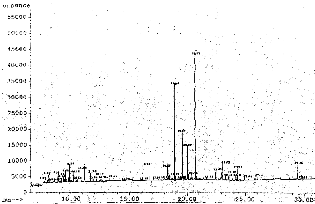
Fig (1.a): GC-MS Chromatogram of volatile compounds of stevia leaves
