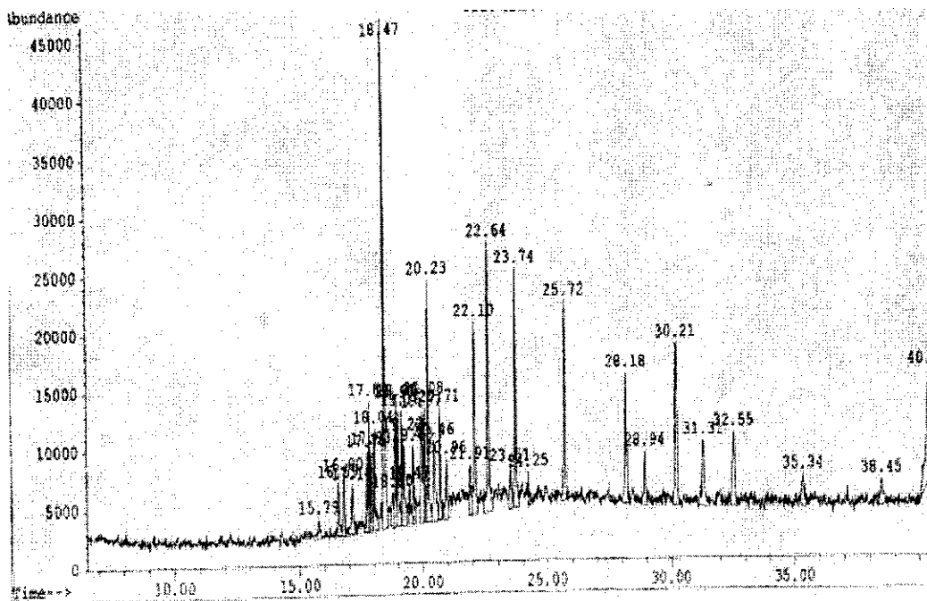
Fig (1.d): GC-MS Chromatogram of volatile compounds of chicory roots
