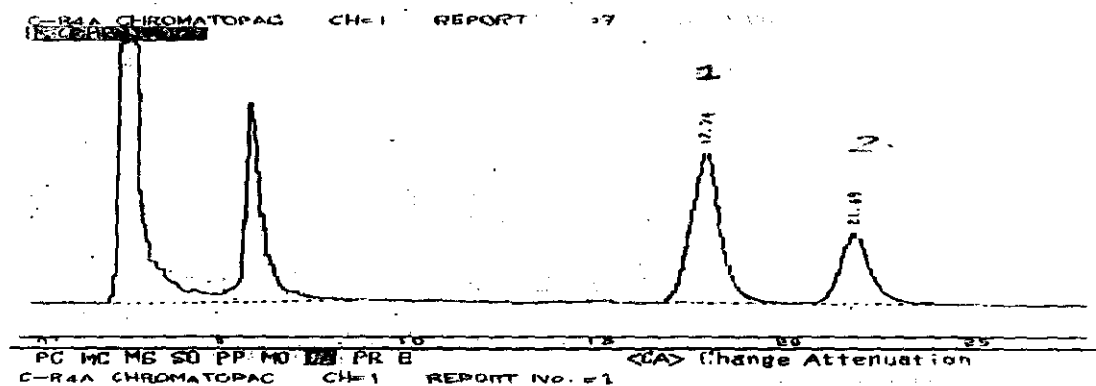
Fig. (1): HPLC-Chromatogram of standard solution consisting of 2 selected biogenic amines.
