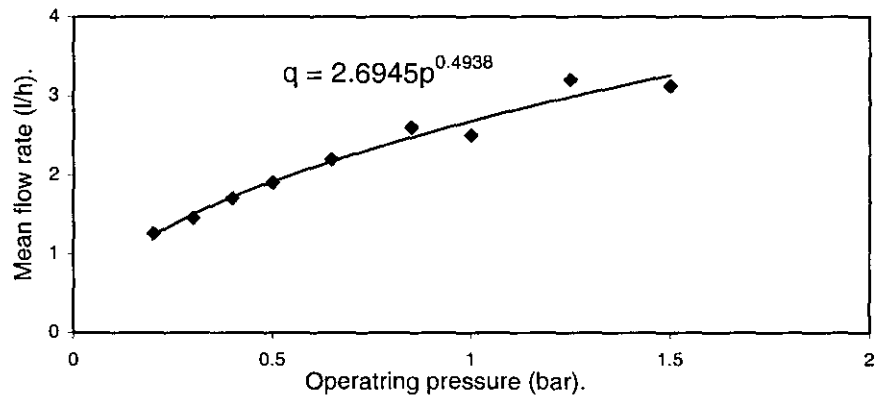
Fig. (4) The relationship between operating pressure and mean flow rate for P.E. O.D. 20 mm.
