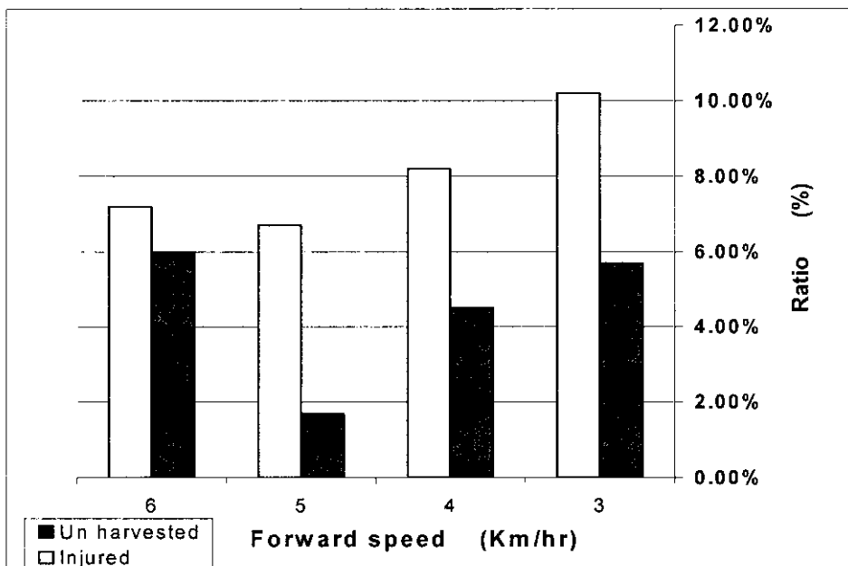
Fig 4. The effect of the forward speed on root losses.
