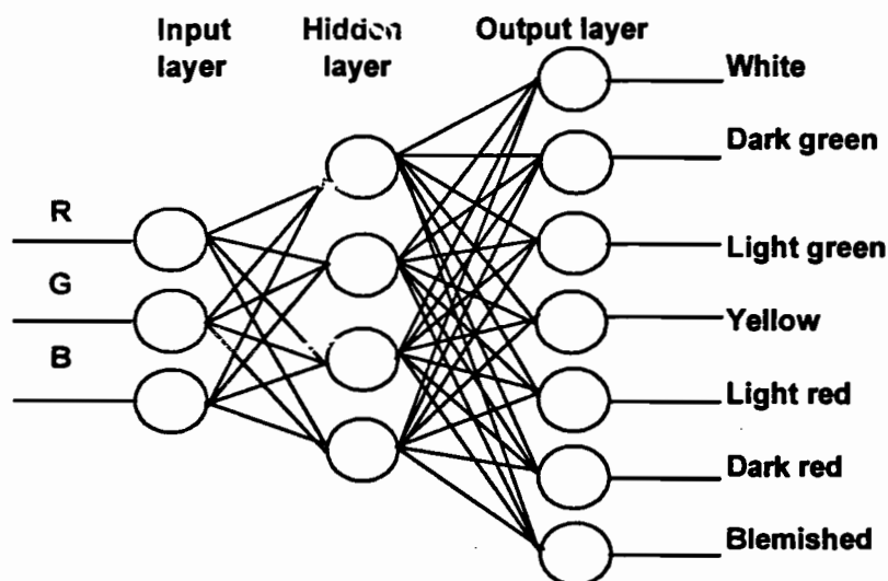
Fig. 6. A typical system of ANN for classified grape
