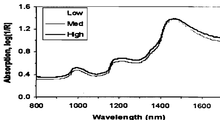
Fig. 9. Average absorption spectra of Superior for three sugar content levels: low (Brix < 11.0 %), medium (11 % < Brix < 16 %), and high (Brix > 16 %). There were 100 fruit for the low class, 250 fruit for medium, and 100 fruit for high
