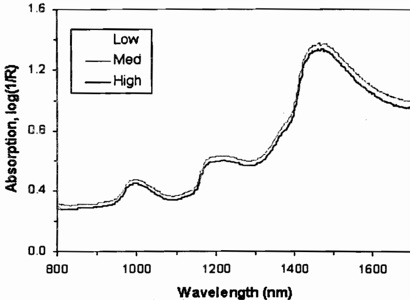
Fig. 7. Average absorption spectra of Superior for three firmness classes as measured by LFRA Texture Analyzer (2mm and 5mm depth) maximum force: low ( F < 3.4 N), medium ( 3.4 \text{ N} < F < 6.2 N), and high ( F > 6.2 N). There were 100 fruit for the low class, 250 fruit for medium, and 100 fruit for high
