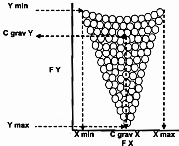
Fig. 5. Shape estimation
