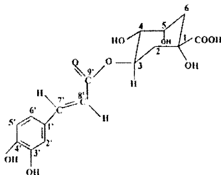
Chlorogenic acid
