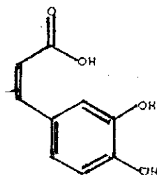
Caffeic acid
