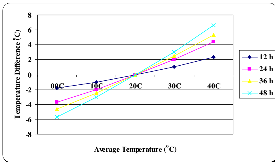
Figure 3: The sensitivity curves with respect to the average air temperature are linear (for all curves, r = 0.99 ). The temperature difference is the difference between the standard and the trials at either 12 hours, 24 hours, 36 hours or 48 hours. The slope of each line represents the model sensitivity to changes in the average air temperature.
