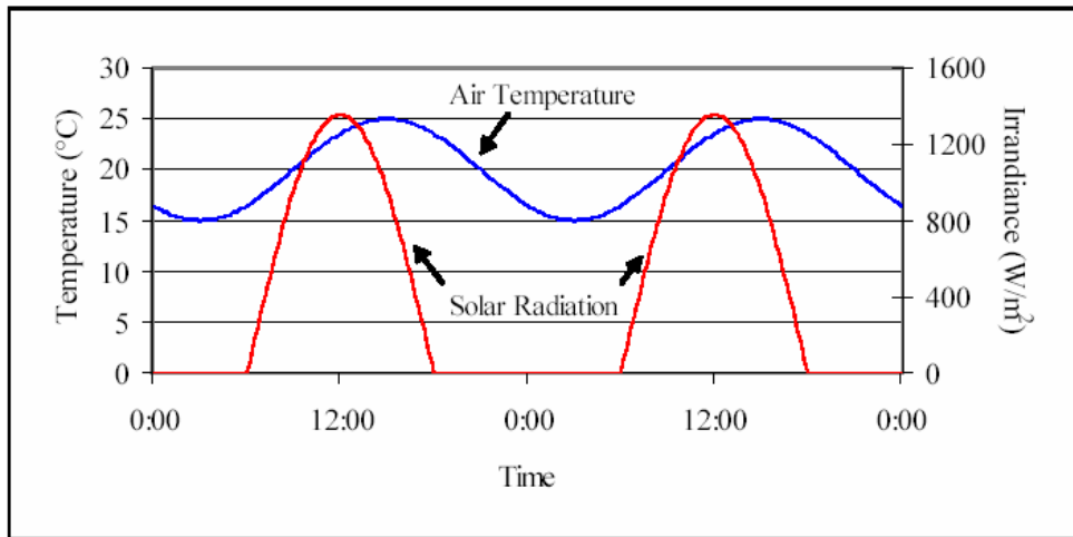
Figure (1): Air temperature and solar radiation were modeled as sinusoidal curves, with a period of one day. At night, solar radiation was held constant at 0 \text{ W m}^{-2} . The air temperature and the solar radiation described by these two curves were used as input data in the sensitivity analysis.
