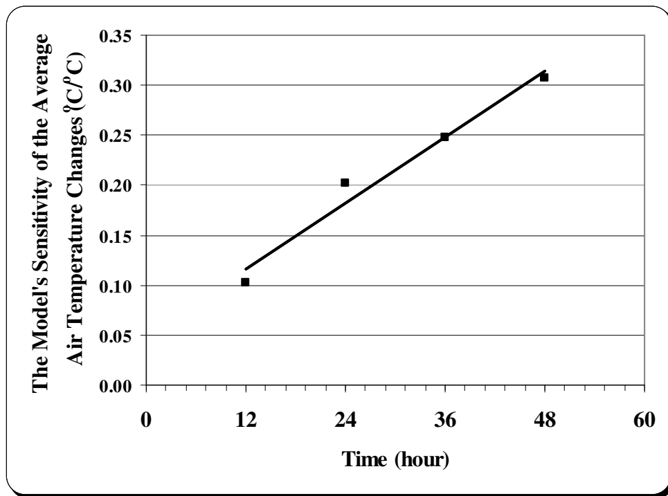
Figure 4: The model's sensitivity to the average air temperature increased with time at a rate of 0.00569 (°C/°C)/hr. The slope of each sensitivity curve was plotted against time to generate this graph.
