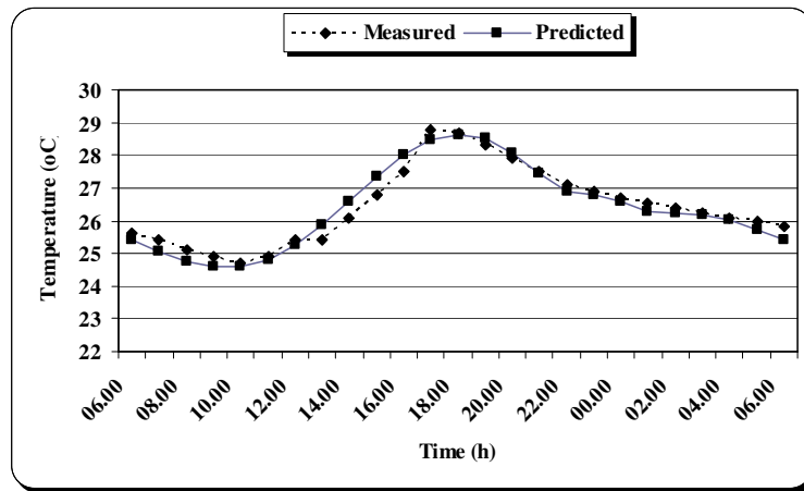
Figure (5): Measured and predicted temperatures.
