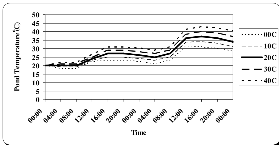
Figure 2: These curves describe how the pond temperature changed over 2 days of hypothetical weather. The temperature labels on the right hand side of the graph were the average air temperature for the sensitivity analysis trials. Cooler air temperatures caused the pond temperature to decrease with respect to the standard (shown here as the 20°C curve). Warmer air temperatures caused the pond temperature to increase with respect to the standard.
