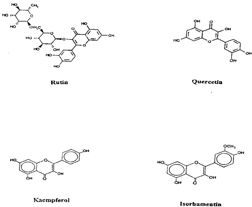
Fig. 1. Chemical structures of investigated flavonoids.
