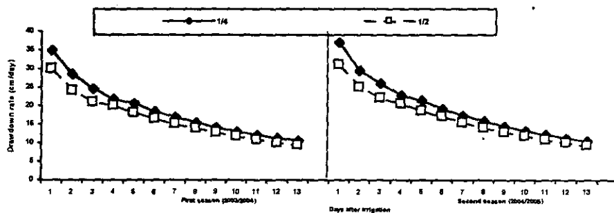
Fig. (1): Average water draw-down rate at 1/4 and 1/2 distance from tile drain under wheat crop in 2003/2004 and 2004/2005 seasons.
