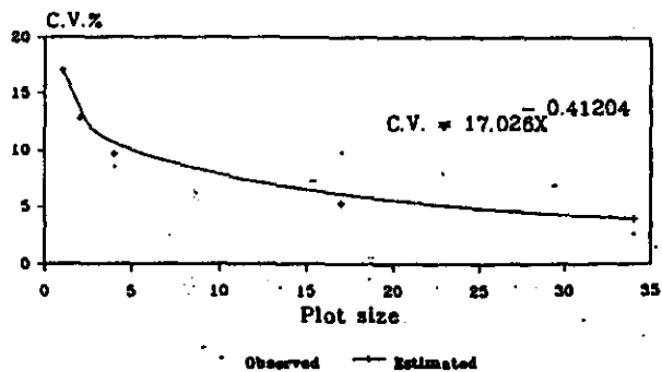
Fig.(1):Relationship between plot size and coefficient of variability(CV)for Giza 2 (control irrigation 2002).
