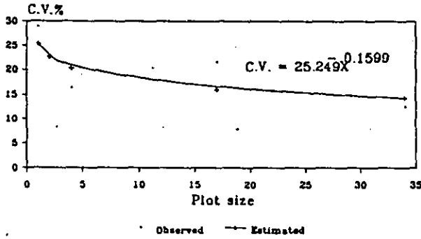
Fig.(7): Relationship between plot size and coefficient of variability(CV)for S.C.10 (stress irrigation 2002).
