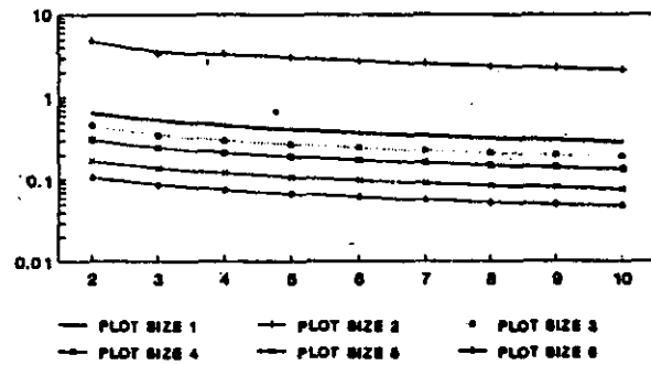
Fig.(16):The relationship between standard error for different plot sizes and various number of replications.
