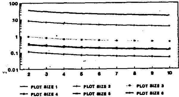
Fig.(12):The relationship between standard error for different plot sizes and various number of replications.
