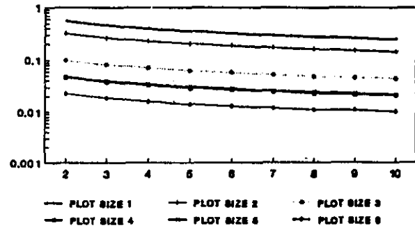
Fig.(14):The relationship between standard error for different plot sizes and various number of replications.
