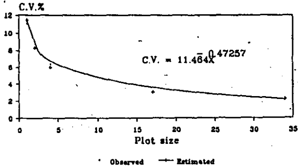
Fig.(5): Relationship between plot size and coefficient of variability(CV)for S.C.10 (control irrigation 2002).
