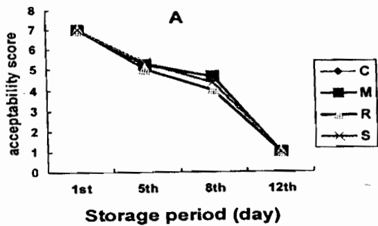
Fig. 5: Overall acceptability scores of minced beef during refrigerated storage
