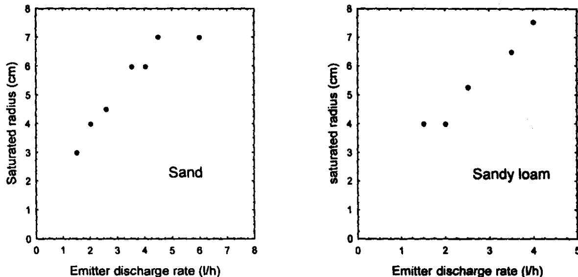
Figure 1. the final saturated radius as related to the emitter discharge rate
