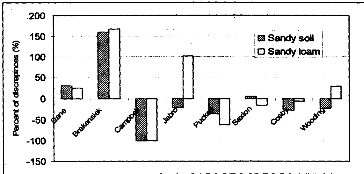
Figure 3. The discrepancies ( in percent) between the several predicted methods (as compared to the constant head method) for predicting saturated hydraulic conductivity for sand and sandy loam soil
