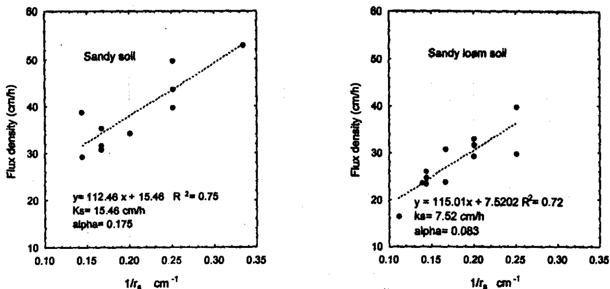
Figure 2. the relationship of flux densities, q , versus the reciprocal of steady-state radii, 1/r_s , for sandy and sandy loam soil.
