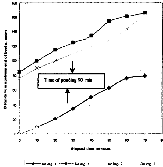
Fig. 3. Irrigated length and elapsed time for C treatment
