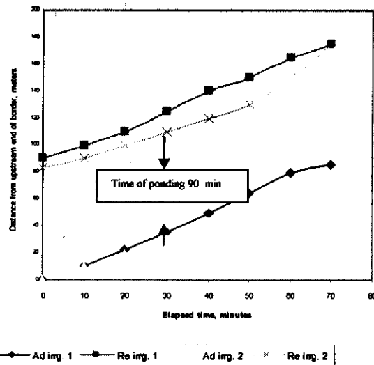
Fig. 2. Irrigated length and elapsed time for B treatment.
