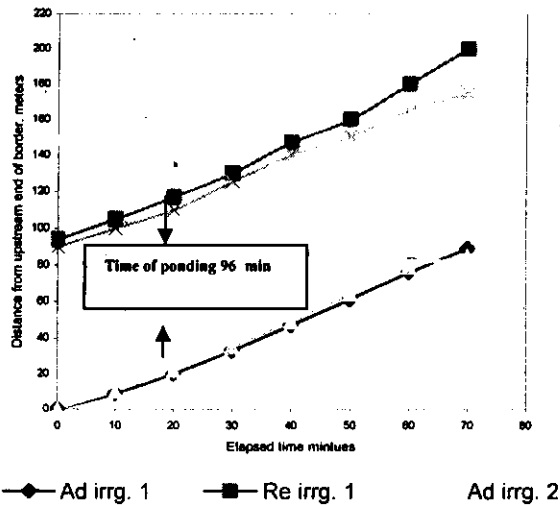
Fig. 1. Irrigated length and elapsed time for A treatment (control). ( Time of ponding = Infiltration opportunity time)
