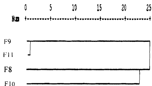
Fig. 8. Dendrogram showing molecular relationship between the four ECM strains (F8, F9, F10 and F11) based on ISSR analysis using Dice Measure
