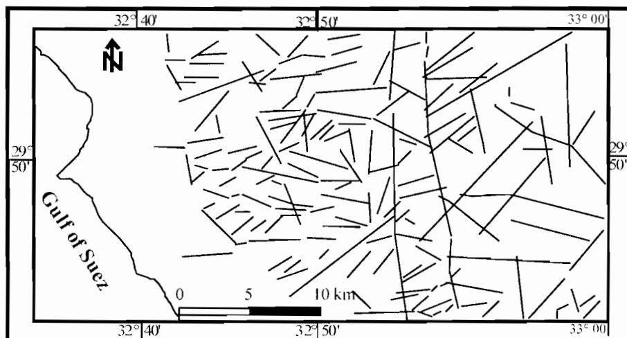
Fig. (5). Structural lineament systems of Ayoun Mousa and adjacent areas.
