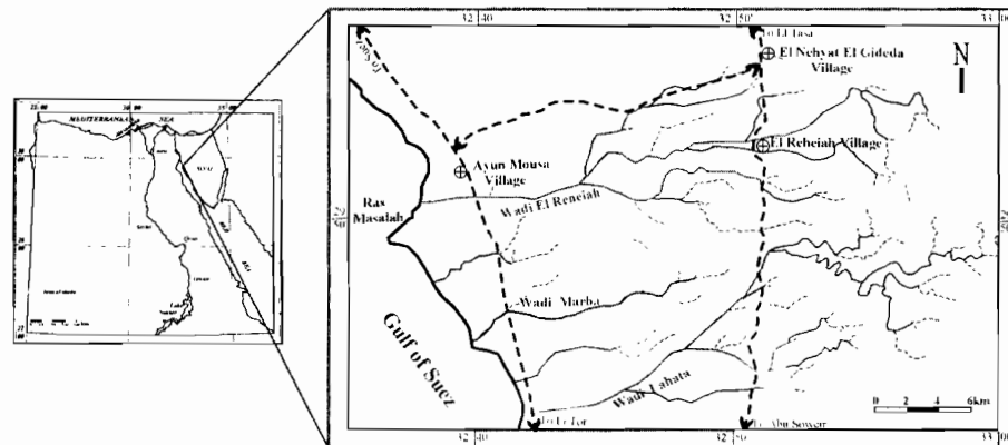
Fig. (1). Location map of Ayoun Mousa and adjacent areas.
