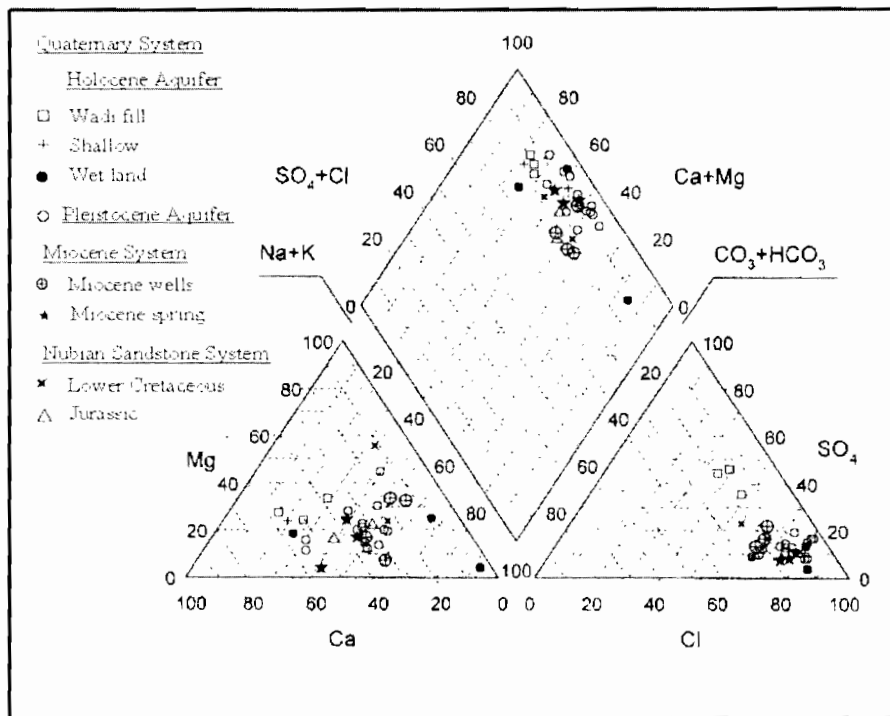
Fig. (9). Genetic classification of water points in the study area.
