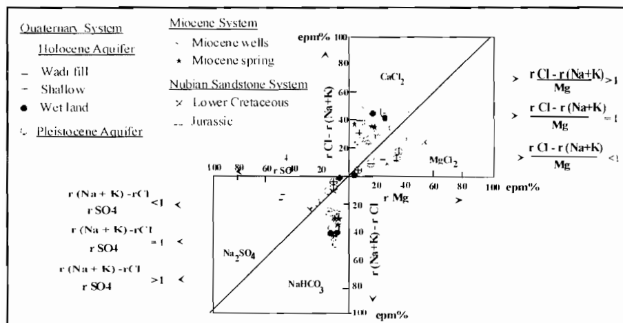
Fig. (10). Sulin Diagram of the study area.
