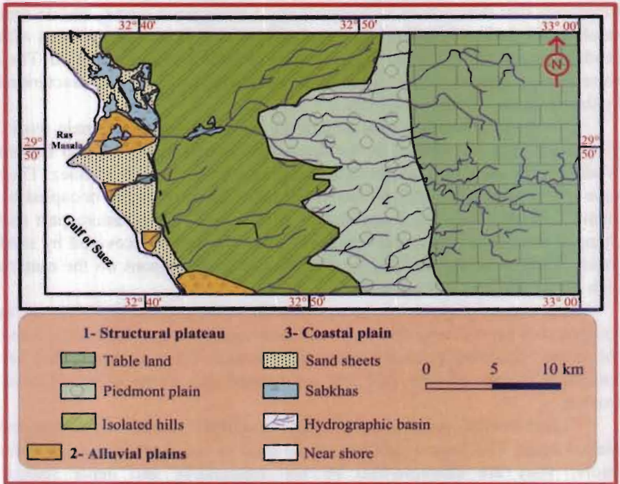
Fig. (2). Geomorphological map of Ayoun Mousa and adjacent areas.
