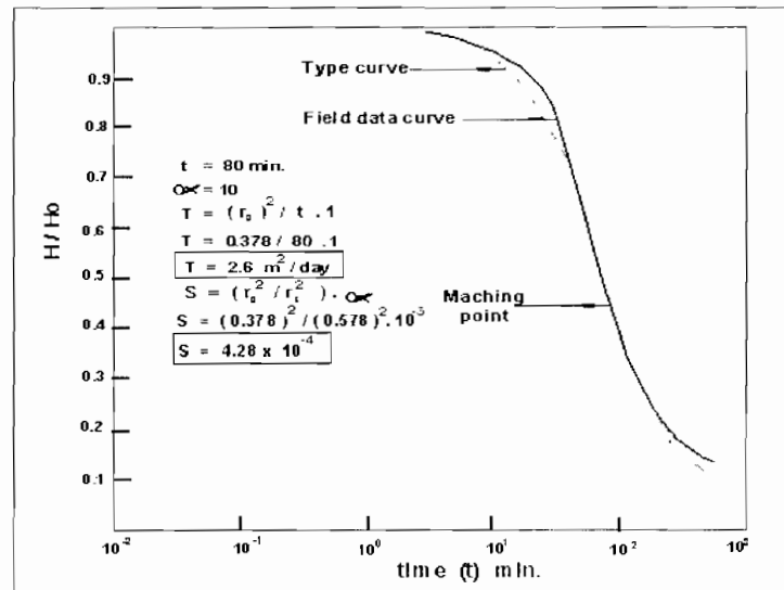
Fig. (5). Analysis of pumping test data of Abu Ramad-2 dug well.
