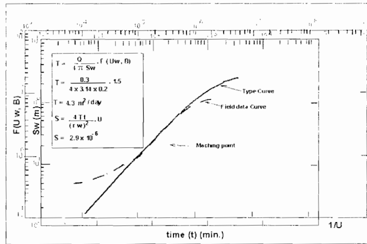
Fig. (4). Analysis of pumping test data of Emblacite well.
