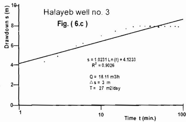
Fig. (6). Analysis of pumping test data of Halayeb wells (1, 2 and 3).
