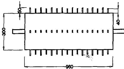
Spike tooth drum 30° {T 3 }
