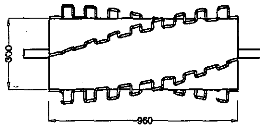
Crank drum 30° {T 1 }
