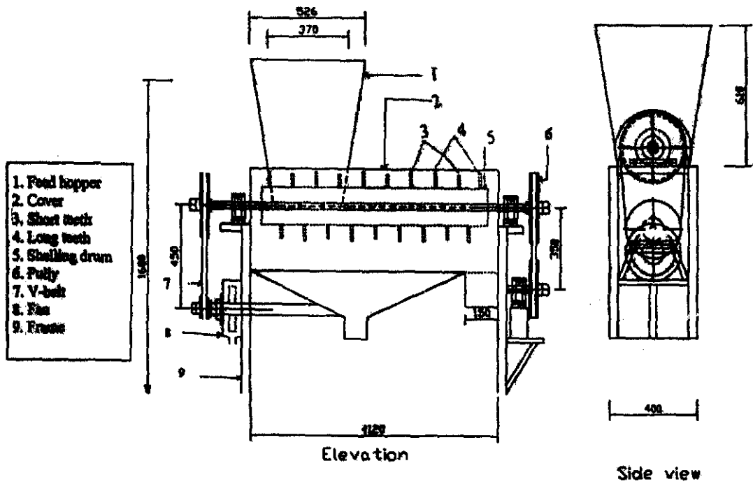
Fig(1) Schematic diagram of shelling corn unit elevation and side view (dim.in mm)
