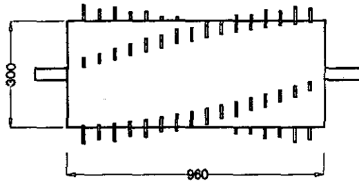
Spike tooth drum 30° {T 2 }
