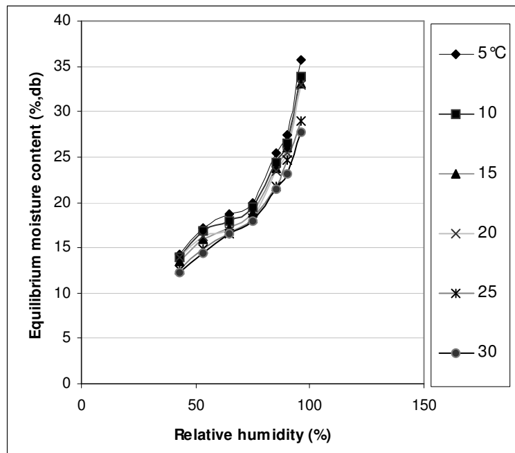
Fig.(1): Equilibrium moisture content for sheep wool materials. The results revealed that the equilibrium moisture content of the sheep wool increased with increasing the relative humidity but it decreased with
