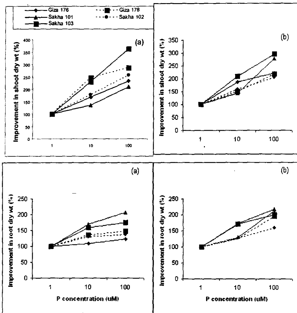
Fig.(2): Improvement in shoot and root dry weight without NaCl (a) and with 50 mol m -3 NaCl (b) of five rice varieties due to substantial increase of phosphorus supply over its minimum concentration.
