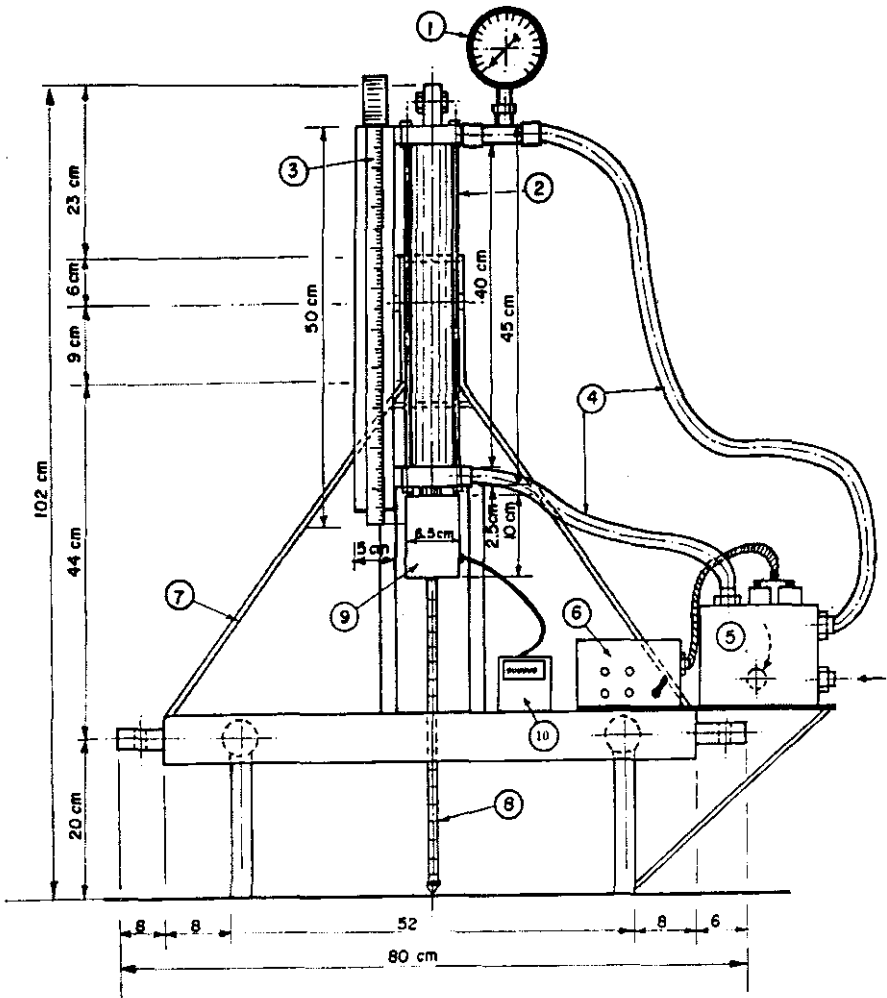
Fig. (3): Schematic diagram of the developed device showing arrangement to collect soil cone index data.
