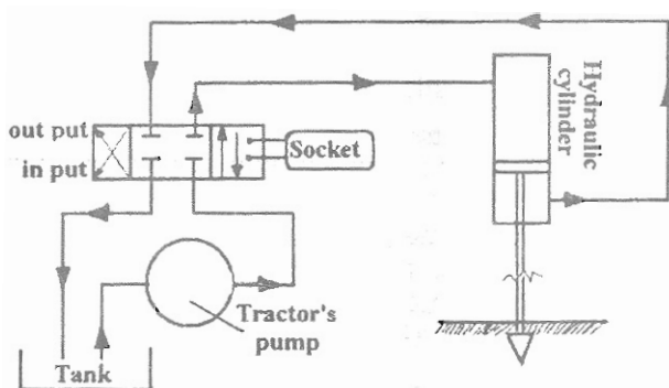
Fig. (7): The hydraulic system connections Laser Alignment (1992).
