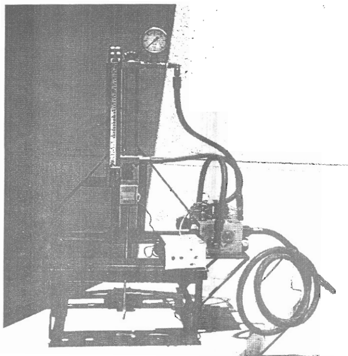
Fig. (4): Photo of the developed device showing arrangement to collect soil cone index data.
