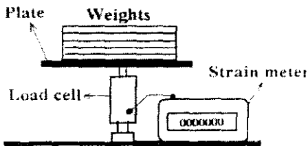
Fig. (9): Calibration set-up for the load cell.
