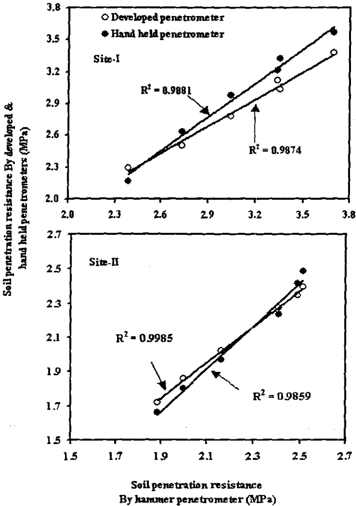
Fig. (11): Variation of soil penetration resistances measured by locally made hammer penetrometer and by both developed and hand held penetrometers.
