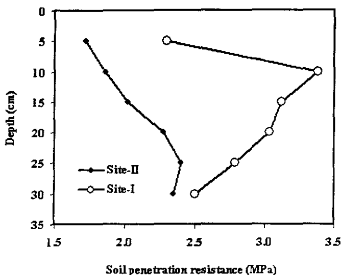
Fig. (10): Means of penetration resistance for site-I and site-II at different depths.
