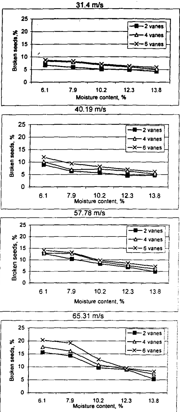
Fig. (7): The effect of seeds moisture content on broken percentage at different number of vanes on spinning disc
