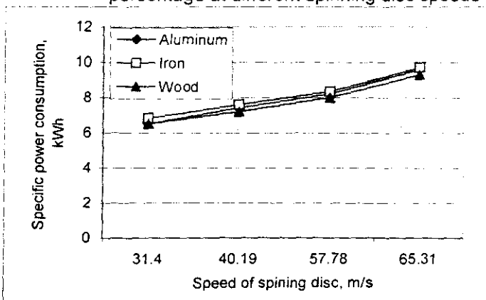
Fig. (10): The effect of spinning disc materials on power consumption at different different spinning disc speeds
