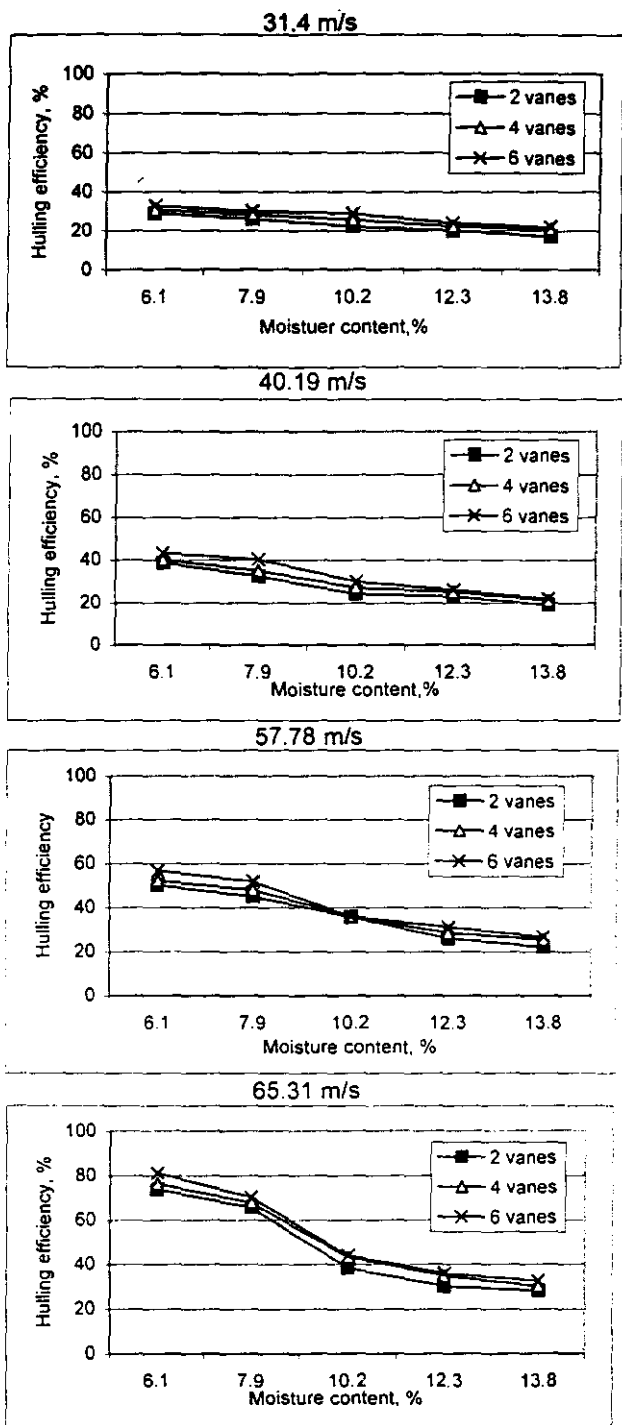
Fig. (5): The effect of seeds moisture content on hulling efficiency at different number of vanes
