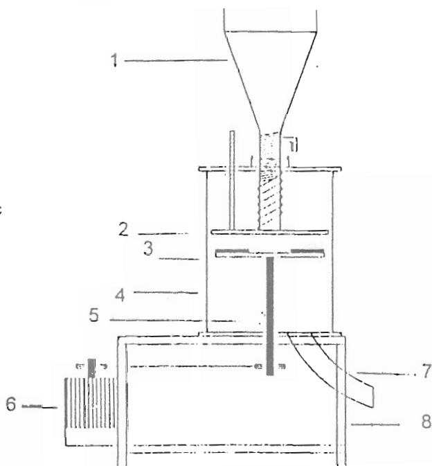
Fig. (3): Sketch of the hulling prototype
