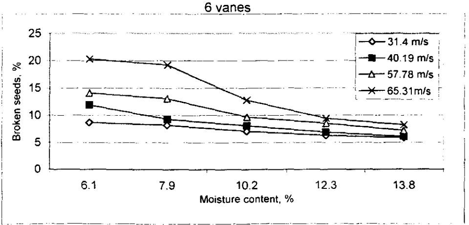
Fig.(6):The effect of seeds moisture content and spinning disc speeds on broken seeds percentage at different number of vanes
