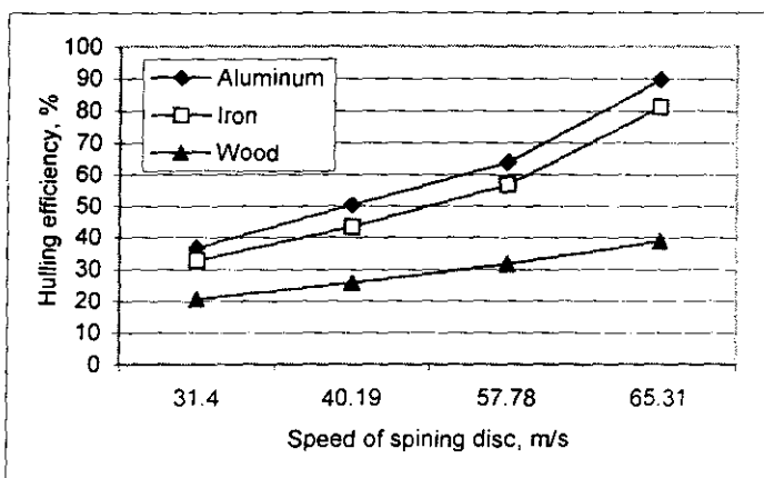
Fig. (8): The effect of spinning disc materials on hulling efficiency at different spinning disc speeds
