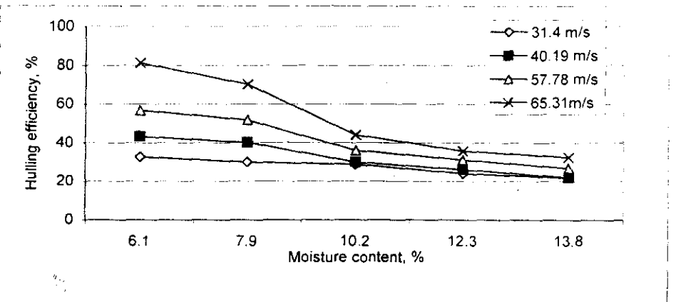
Fig.(4): The effect of seeds moisture content on hulling efficiency at different spinning disc speeds and different number of vanes
