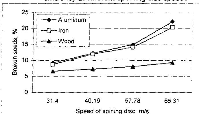
Fig. (8): The effect of spinning disc materials on hulling efficiency at different spinning disc speeds
