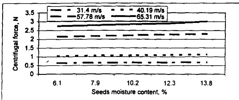
Fig. (1): The theoretical hulling force (centrifugal) at different speeds and seeds moisture content Iron spinning disc
