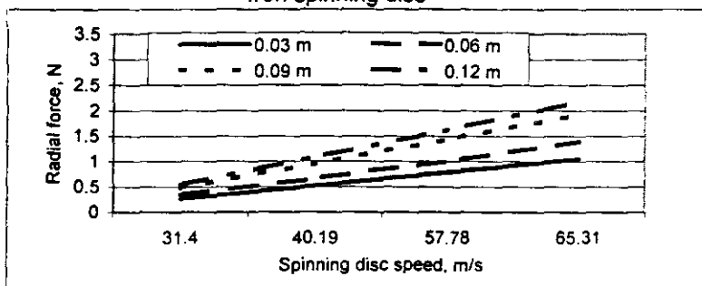
Wood spinning disc
