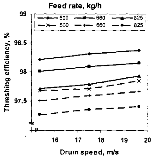
Fig 7: Effect of drum speed on threshing efficiency under different feed rates at different moisture contents.
