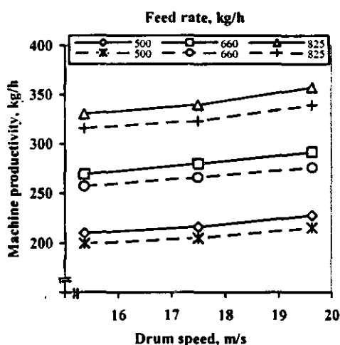
Fig 3: Effect of drum speed on machine productivity under different feed rates at different moisture contents.
