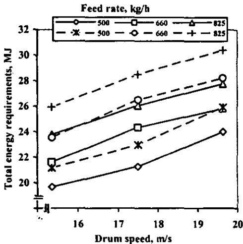
Fig. 4: Effect of drum speed on total energy requirements under different feed rates at different moisture contents.
