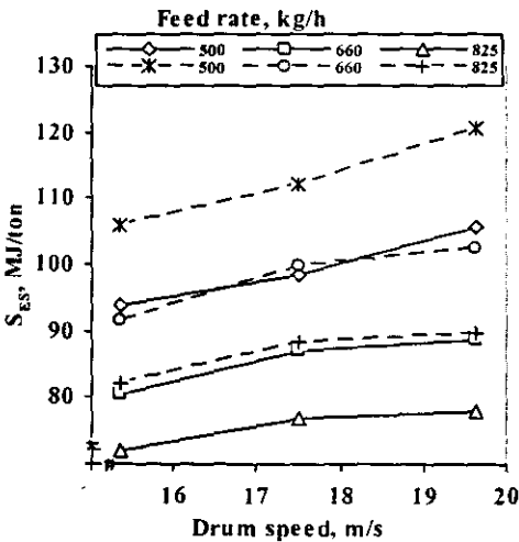
Fig 6: Effect of drum speed on S_{ES} under different feed rates at different moisture contents.
