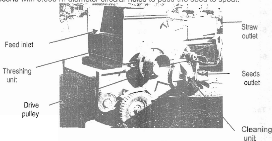
Fig. 1: Threshing machine.
