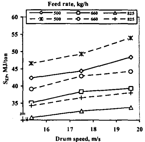
Fig 5: Effect of drum speed on S_{EP} under different feed rates at different moisture contents.
