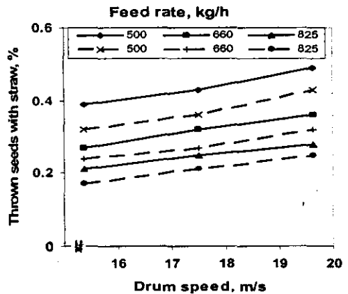
----- = Mc 14.91 % Fig 9: Effect of drum speed on thrown seeds with straw under different feed rates at different moisture contents.
