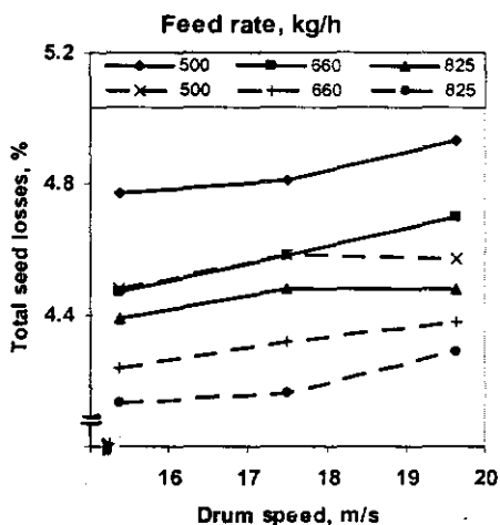
Fig 10: Effect of drum speed on total seed losses under different feed rates at different moisture contents.
