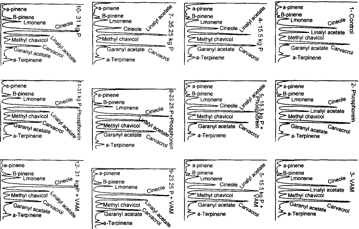
Figure (1): Effect of mineral and bio-phosphate fertilizers and their combination on the essential oil components (%) of marjoram plant during 2005 season.
