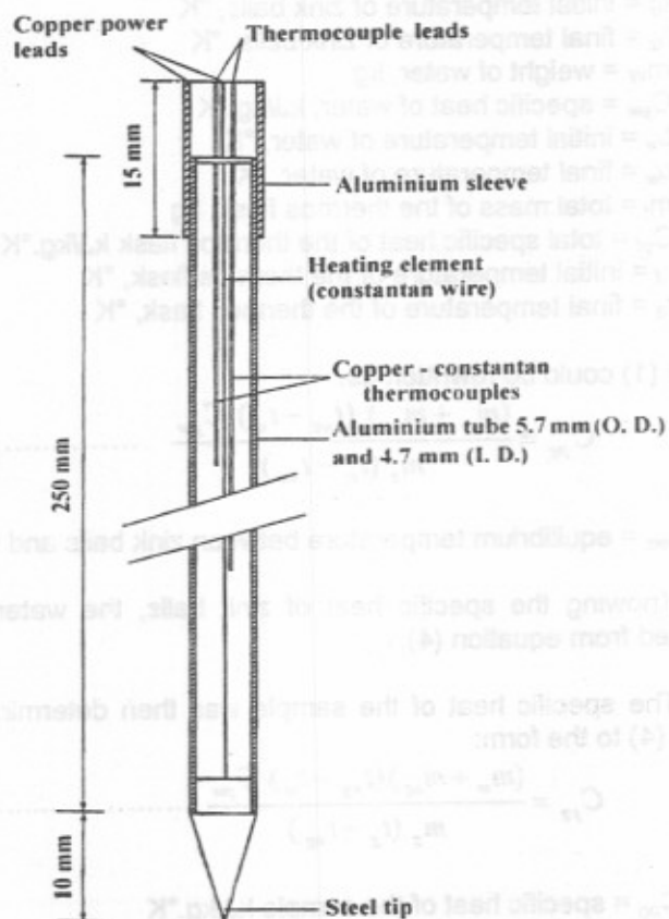
Fig. (4): Thermal conductivity probe
