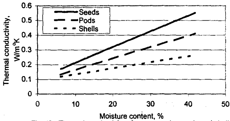
Fig. (6): Thermal conductivity of peanut pods, seeds and shells at different levels of moisture content
