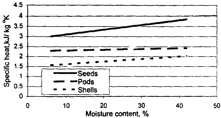
Fig. (5): Specific heat of peanut pods, seeds and shells at different levels of moisture content
