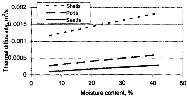
Fig. (7): Thermal diffusivity for peanut pods, seeds and shells at different levels of moisture content
