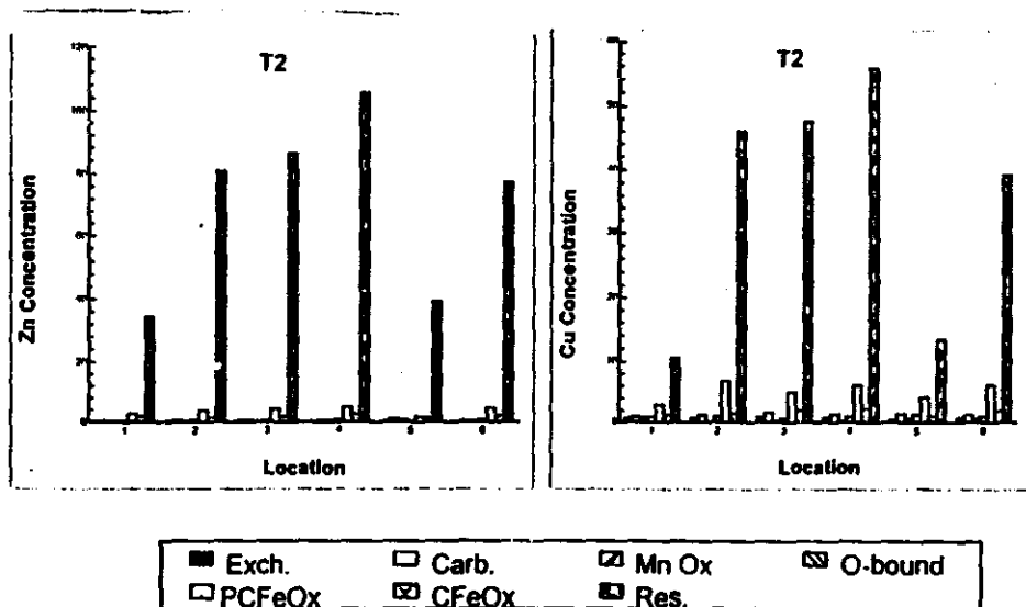
Fig.3: Zinc and Cu forms (mg/kg) in the studied soils of Transect 2.
