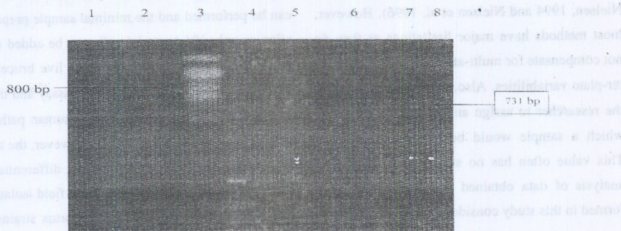
Figure (2): Agarose gel electrophoresis of PCR products obtained with brucella genomic DNA using B. melitensis specific primers
