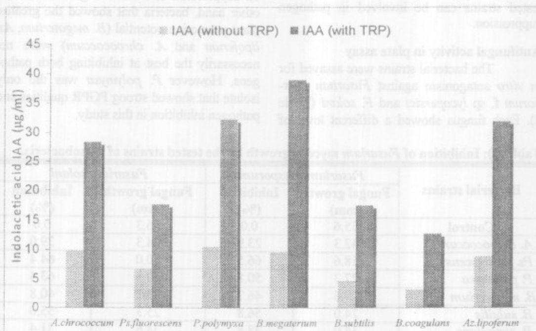
Fig. (2): Indolacetic acid produced from selected rhizobacteria (with and without tryptophan TRP)
