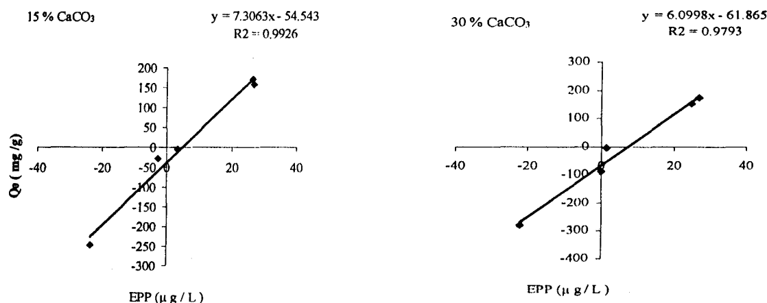
Fig. 1. Phosphorus quantity – intensity relation ship in both tested calcareous soils
