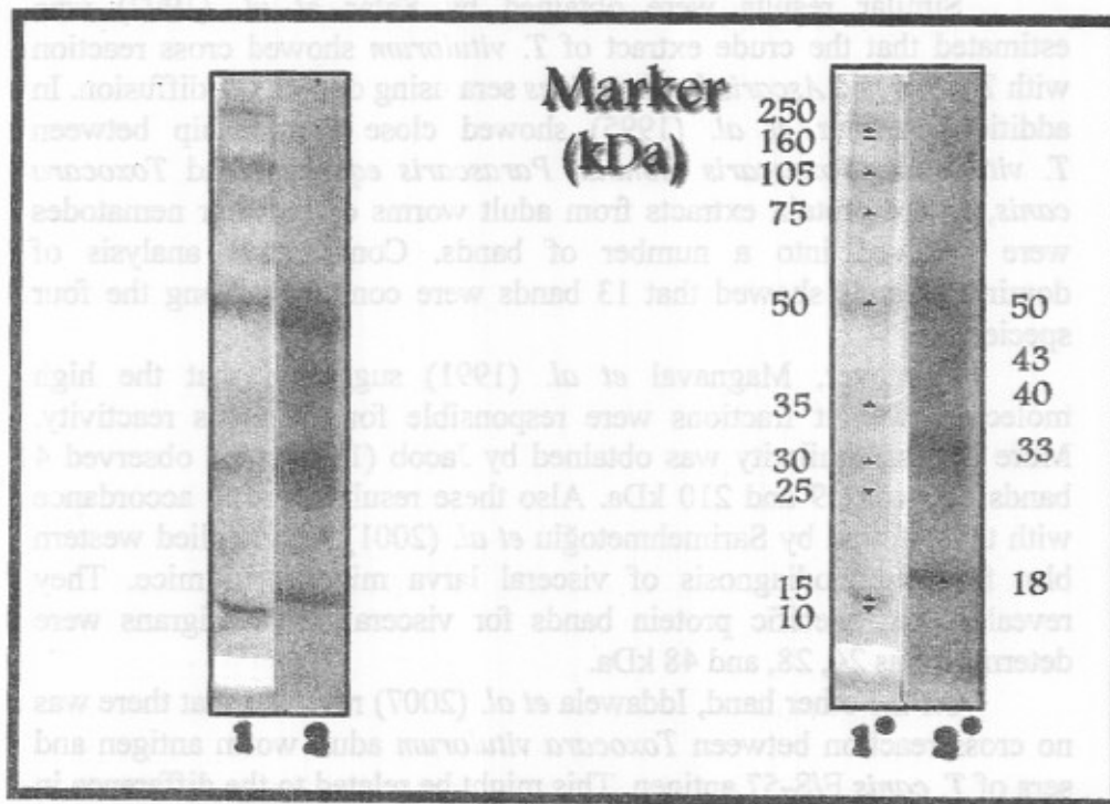
Plate 1: The common epitopes revealed from the reaction of T. vitulorum egg antigen with sera of both T. vitulorum and T. canis (1, 1*: Marker)
