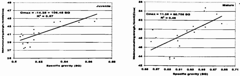
Fig. 6. Relationship between maximum crushing strength ( C_{max} ) and specific gravity (SG).
