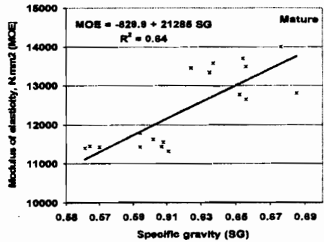
Fig. 5. Relationship between modulus of elasticity (MOE) and specific gravity (SG).
