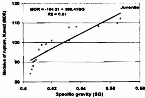
Fig. 4. Relationship between modulus of rupture (MOR) and specific gravity (SG).
