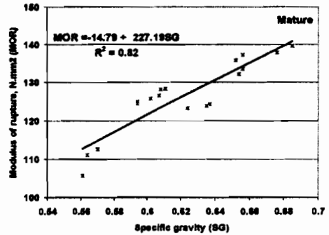
Fig. 4. Relationship between modulus of rupture (MOR) and specific gravity (SG).
