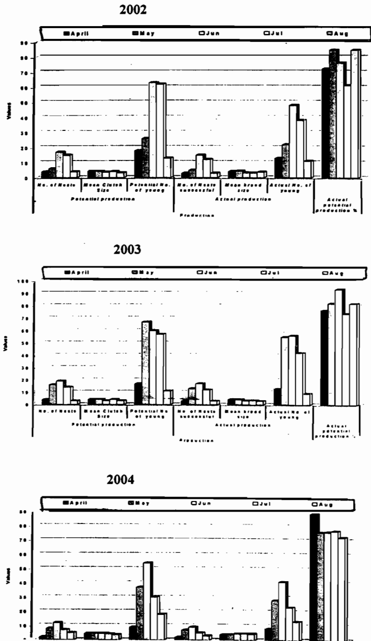
Fig. (1): The actual production compared with potential production of Crested lark Galerida cristat nigricans during 2002, 2003 and 2004.
