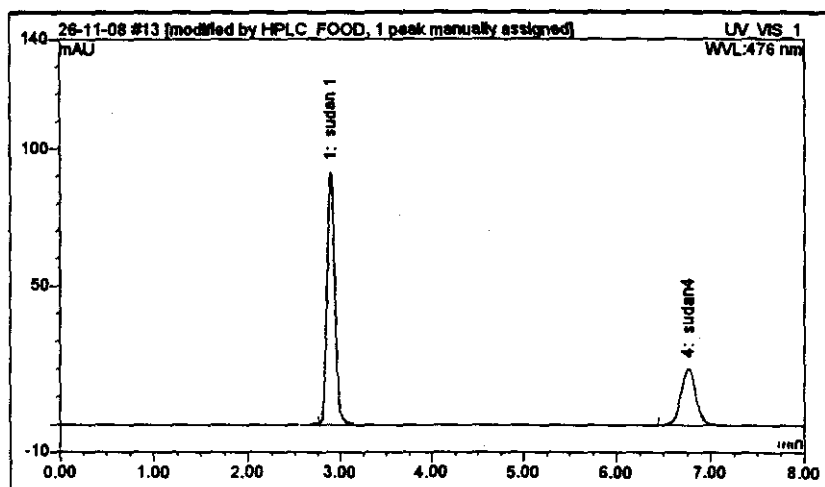
Fig (2): Chromatogram of a SI and S IV dyes detected in one hot chilli powder sample.
