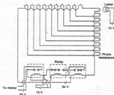
Figure (4): The electronic circuit of sample weight.
