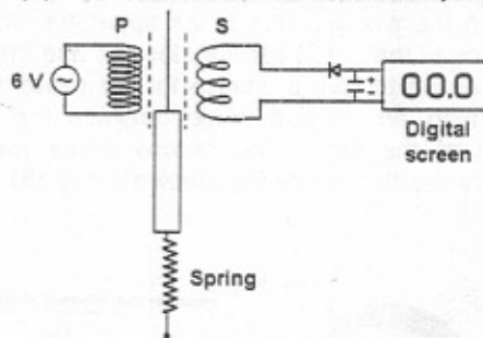
Figure (5): The electronic circuit of friction angle display.
