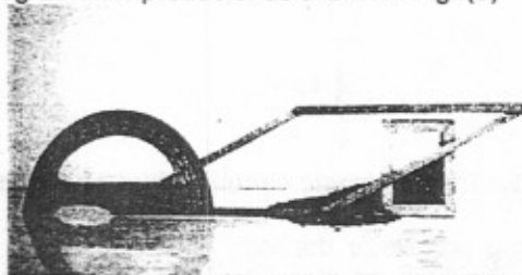
Figure (6): The transparent box and the wooden parallelogram used for measuring the repose angle.
