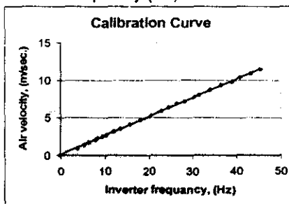
Figure (2): Calibration curve for the terminal velocity apparatus.
