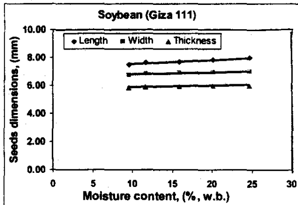
Figure (3): Effect of moisture content on soybean seeds length, width and thickness.
