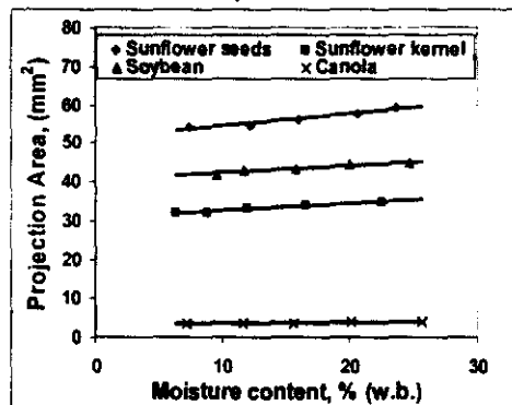
Figure (8): Effect of moisture content on projection area of different studied crops.
