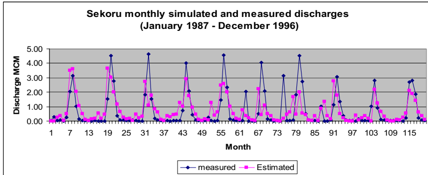
Figure 7 Simulation and measured discharges of Sekoru subwatershed
