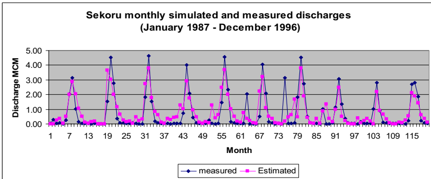
Figure 4 Calibrated discharges of Sekoru subwatershed
