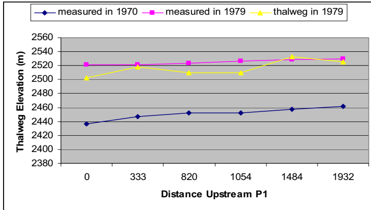
Figure 6 Calibration of the thalweg of Legedadi reservoir
