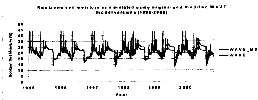
Figure 6: Soil moisture content in the rootzone using original and modified WAVE model versions (1995-2000).
