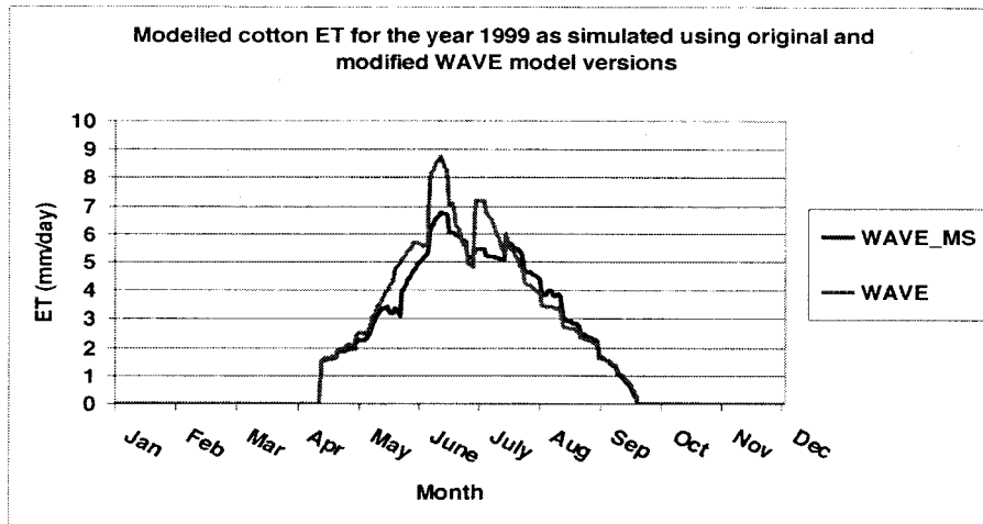
Figure 3- Modelled cotton ET using original and modified WAVE model versions (1999)
