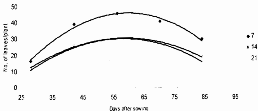
Fig.(1): Number of leaves per plant of sesame with time as affected by irrigation intervals (7, 14 and 21 days) grown during the 2003/04 (a) and 2004/05 (b) seasons in Northern Sudan.
