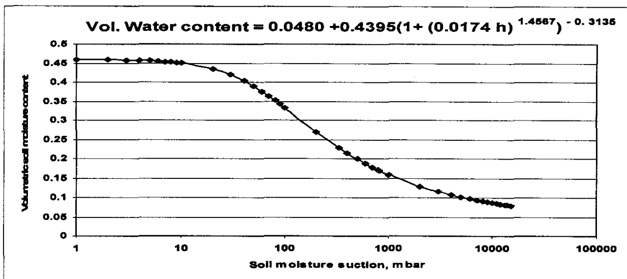
Fig. 1. Soil moisture retention curve of the soil under study
