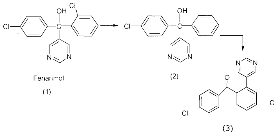
Scheme (1): Main reaction pathways of Fenarimol (According to Mateus et al,2000)
