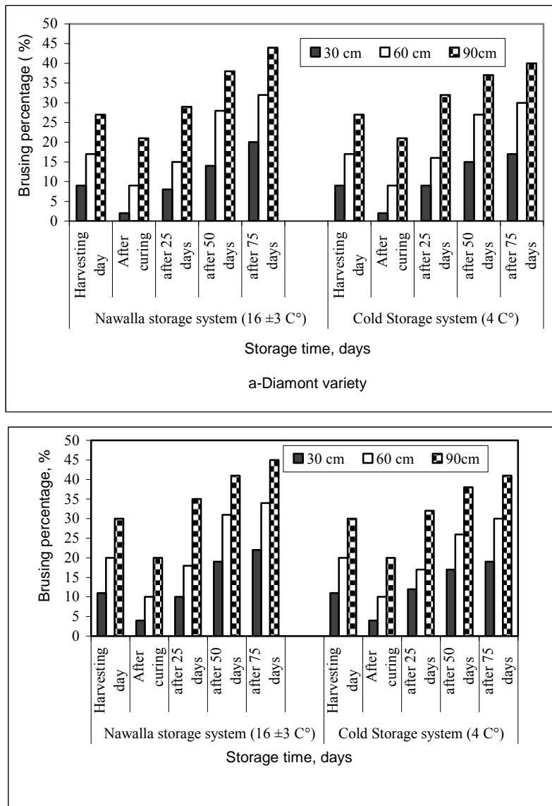
Figure (8): Bruising percentage of potato tubers due to impact height for fresh tubers; after 15 days curing period and during the storage of tubers in Nawalla and Cold storage systems for a-Diamont and b-Santana varieties.
