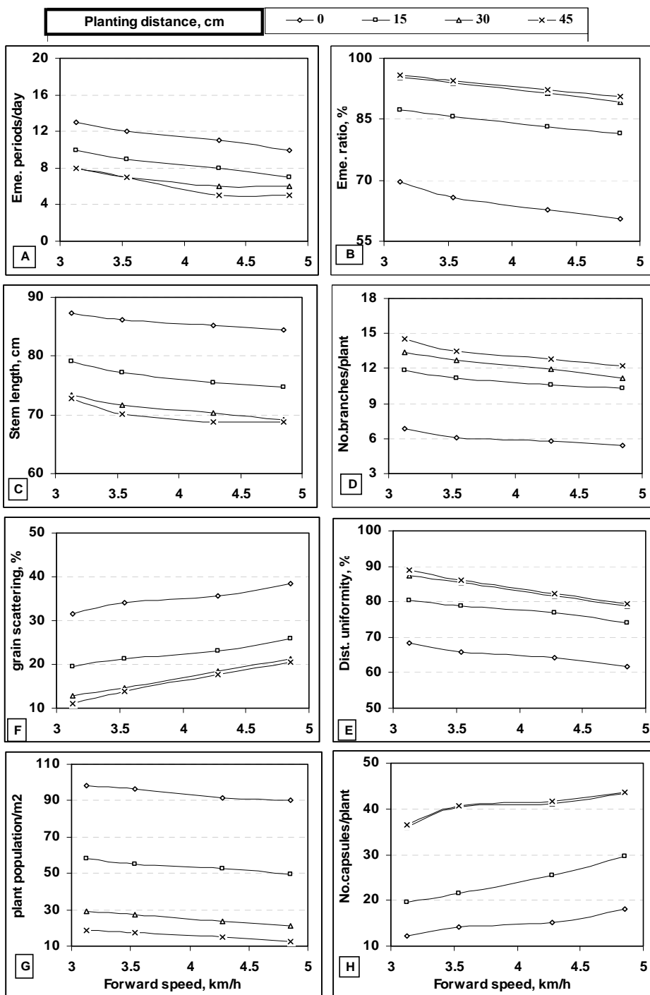
Fig. (6): Effect of the distance between plants and forward speed of developed seed drill on some physical characteristics of ' black seed' plants.
