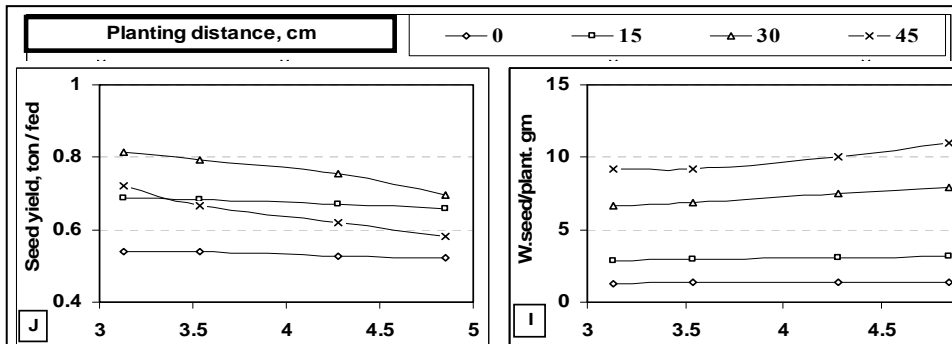
Fig. (6)cont.: Effect of the distance between plants and forward speed of developed seed drill on some physical characteristics of ' black seed' plants.
