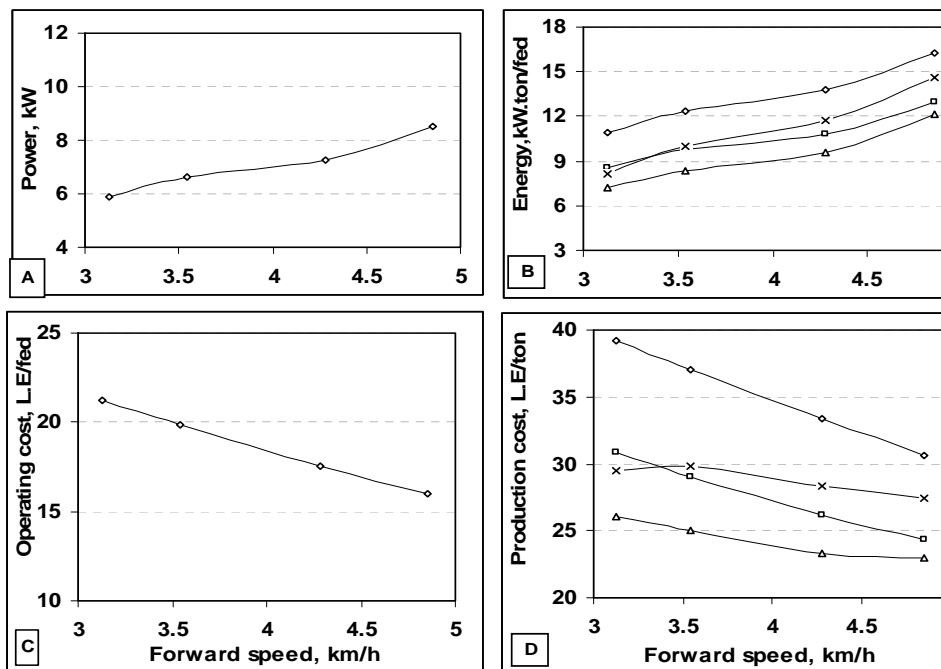
Fig. (8): Effect of the distance between plants and forward speed of developed seed drill on energy requirement production cost
